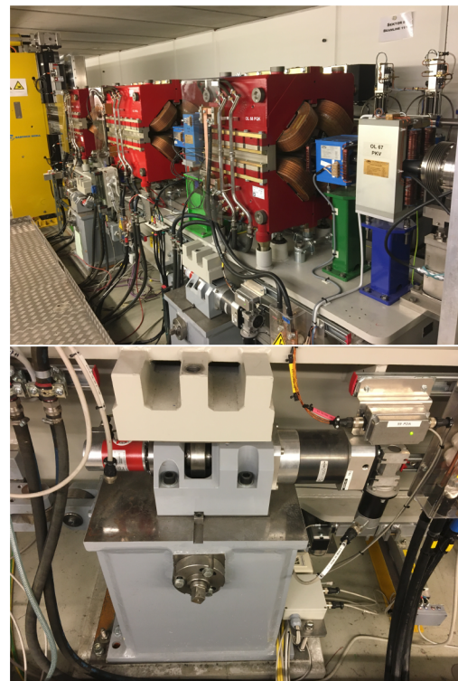
Figure 1: Top: View of a girder installed in the PETRA III tunnel downstream of an undulator (yellow element on the left), carrying three quadrupole magnets. Bottom: Zoom to a motor and encoder installed on the cam mover-based alignment system connecting the supporting feet to the girder table.
