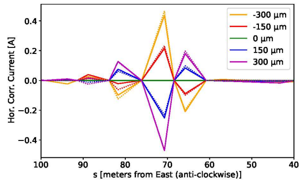
Figure 4: Measured (solid) and simulated (dotted) horizontal corrector currents for the five girder positions as a function of the corrector location counted from the East symmetry point in anti-clockwise direction. Corrector magnets are displayed as small dark blue elements in Fig. 2. Values are given relative to the original girder position.
