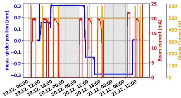
Figure 3: Time evolution over the three-day experiment. The left axis (blue) shows the measured horizontal girder position, the right axes display the beam (red) and dipole magnet (orange) currents, showing the time periods during beam operation and tunnel access for girder movement. Gray shaded areas indicate night time, with magnet current on, but no circulating beam.
