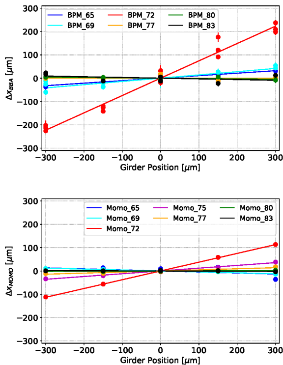
Figure 5: Horizontal beam-based alignment (BBA) data (top) and beampipe position measured with the HF-Movement Monitors (HF-MOMO) (bottom) as a function of the girder position. Lines show the measurement at different locations in the proximity of the moved girder, numbers in the legend labels indicate locations according to Fig. 2.
